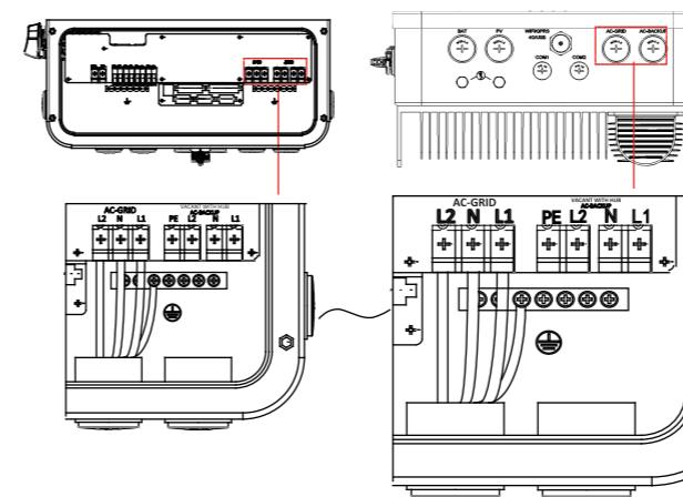
Inverter
